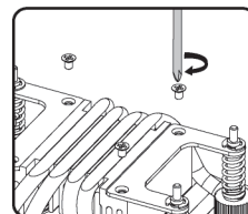
Assemble the AMD AM2/AM2+/AM3 retention bracket mounting kit (D)(E)
