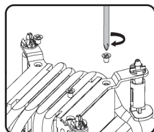
Assemble the Intel LGA 1366 retention bracket mounting kit (B)(E)
